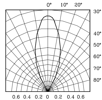
Figure10.Directivity
